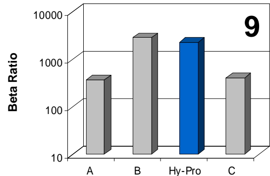
Time Weighted Beta Ratio Comparison per ISO16889 multi-pass for \beta_{5\mu_{[c]}} > 200 or 1000 filter element.
